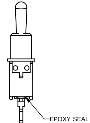
EPOXY SEAL
