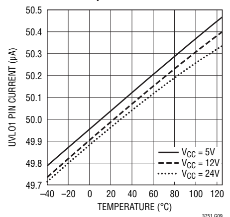
UVLO1 Trip Current
