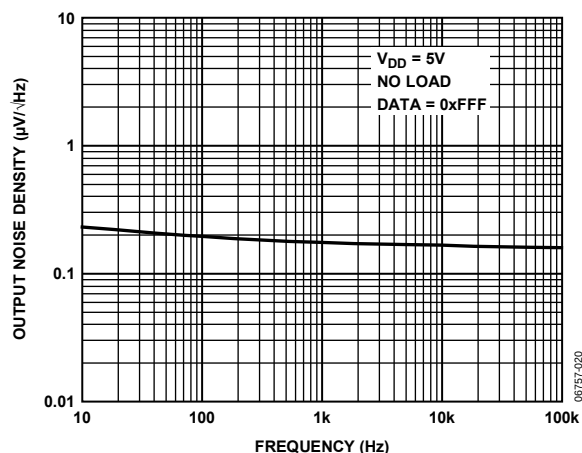
Figure 20. Output Voltage Noise vs. Frequency
