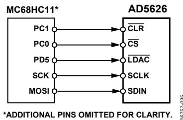
Figure 35. AD5626 to MC68HC11 Interface
