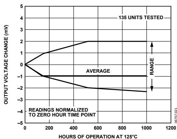
Figure 21. Long-Term Drift Accelerated by Burn-In
