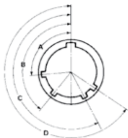
Viewed from front face of receptacle
