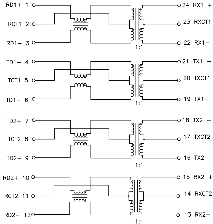
SCHEMATIC
