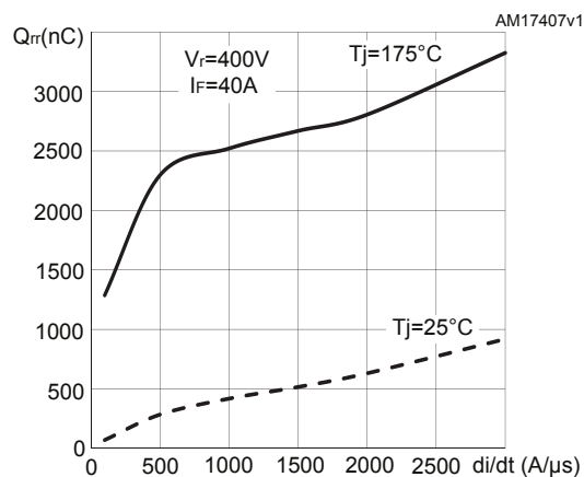
Figure 27. Reverse recovery charge vs diode current slope
