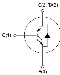
TO-3PF
