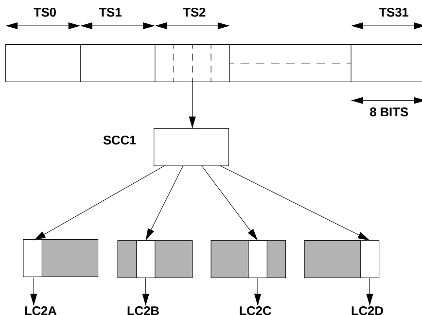
Figure 9-2. Two-Bit Subchannel Implementation with MSC Microcode
