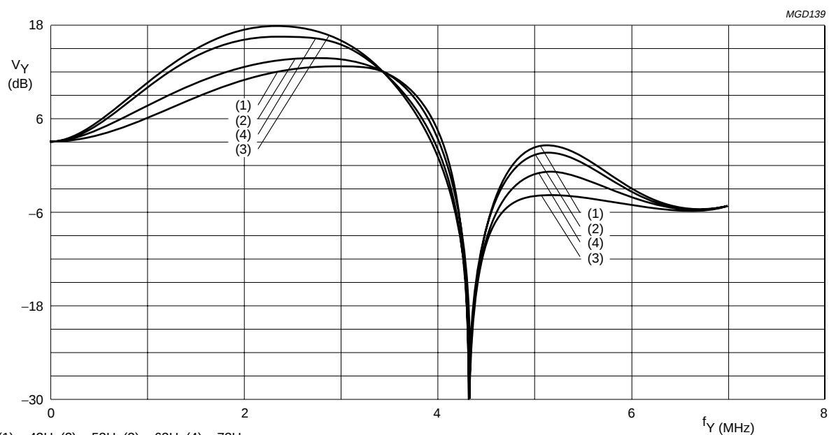
Fig.43 Luminance control SA 09H, 4.43 MHz Trap/CVBS mode, prefilter on, different aperture bandpass centre frequencies.
