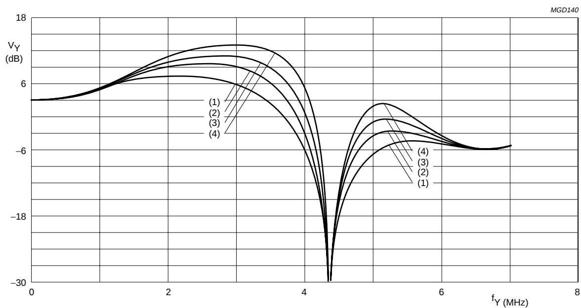
Fig.44 Luminance control SA 09H, 4.43 MHz Trap/CVBS mode, prefilter on, different aperture factors.
