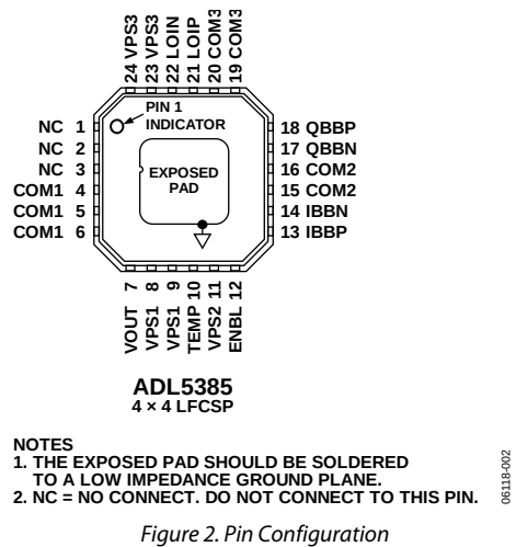
Figure 2. Pin Configuration
