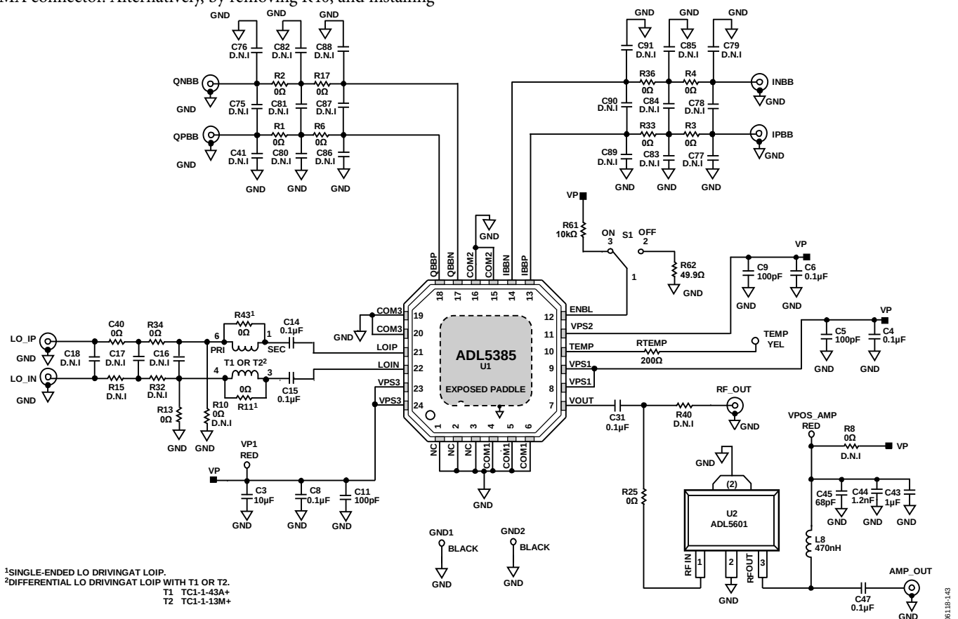
Figure 43. ADL5385-DIFFLO-EBZ Schematic
