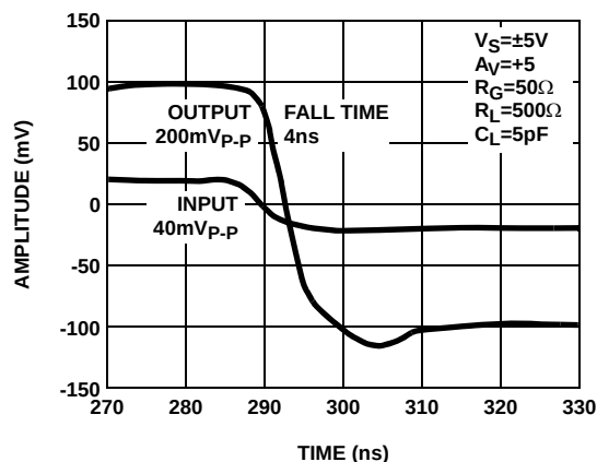
FIGURE 30. SMALL SIGNAL PULSE RESPONSE/FALL TIME
