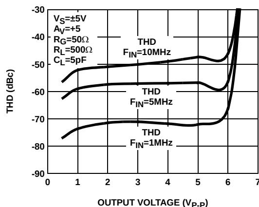
FIGURE 26. THD vs OUTPUT VOLTAGE (WORST HARMONIC)
