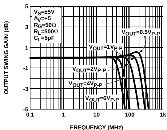
FIGURE 28. OUTPUT SWING vs FREQUENCY
