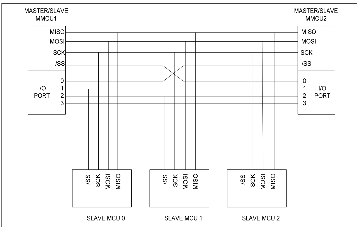
Figure 18-12: SPI multi-master slave environment
