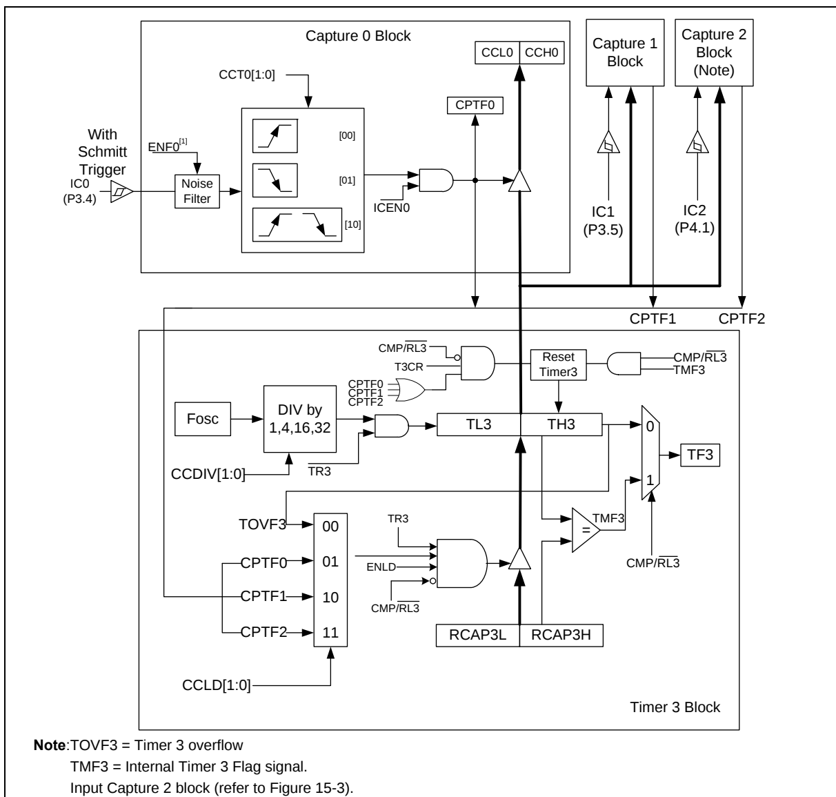
Figure 15-2: Timer3/Capture/Compare/Reload modules
