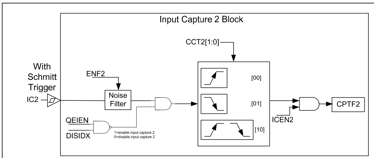
Figure 15-3: Input Capture 2 block diagram
