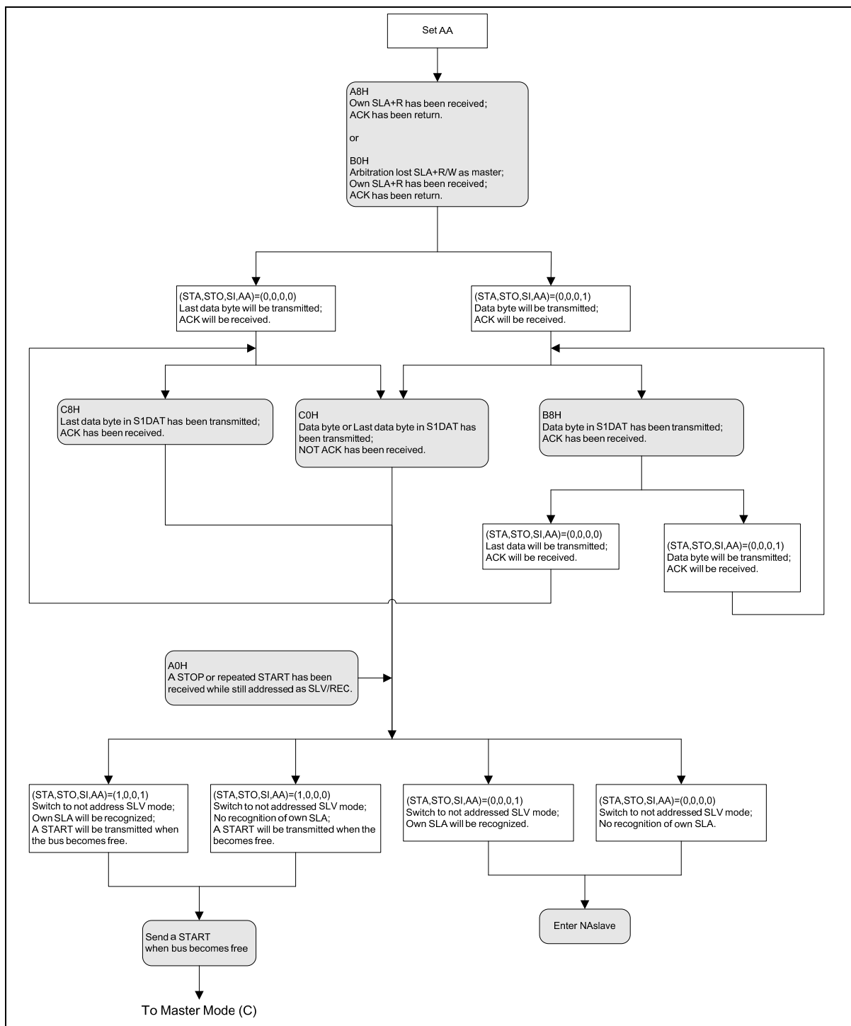
Figure 17-7: Slave Transmitter Mode
