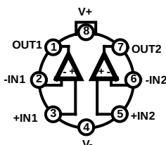
HA-5102 (METAL CAN) TOP VIEW
