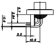
4 : Right angle PCB with brackets and boardlocks
