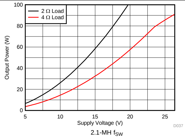
Figure 32. Output Power vs Voltage
