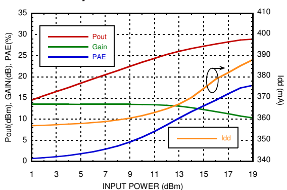
Power Compression @ 22 GHz
