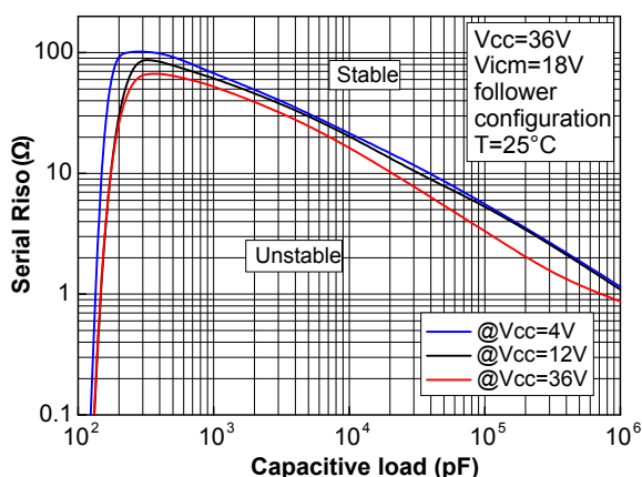
Figure 37. Stability criteria with a serial resistor at different supply voltages
