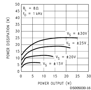
Power Dissipation vs Power Output
