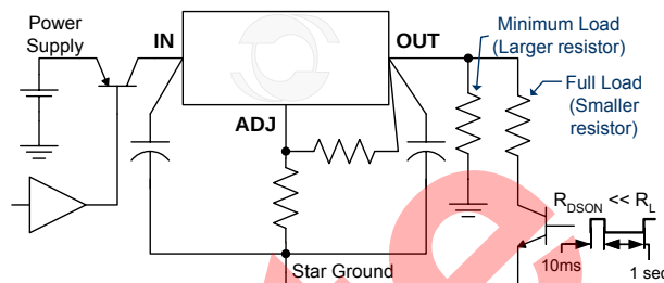
FIGURE 1 - DYNAMIC INPUT AND OUTPUT TEST
