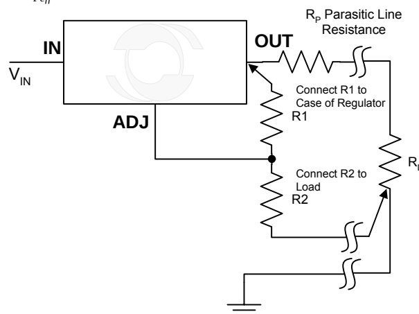
FIGURE 3 - CONNECTIONS FOR BEST LOAD REGULATION
