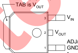
DT PACKAGE (3-PIN) (Top View)
