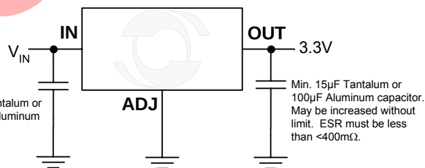
FIGURE 7 - FIXED 3.3V OUTPUT REGULATOR
