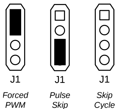
Figure 1. J1 Jumper Setting
