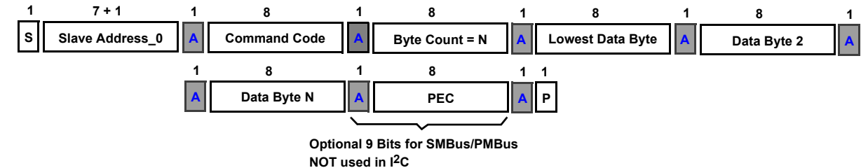
FIGURE 23. SMBus/PMBus/I 2 C COMMAND PROTOCOL
