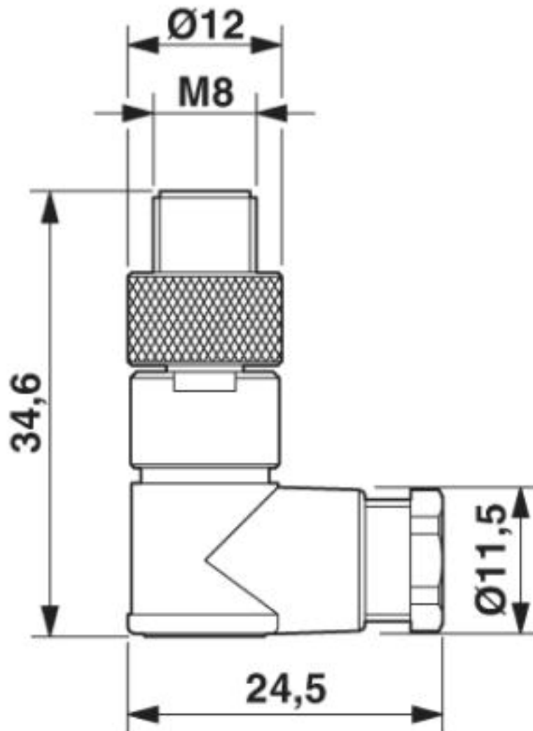
Dimensional drawing
