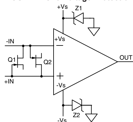
FIGURE 7. Overvoltage Protection
