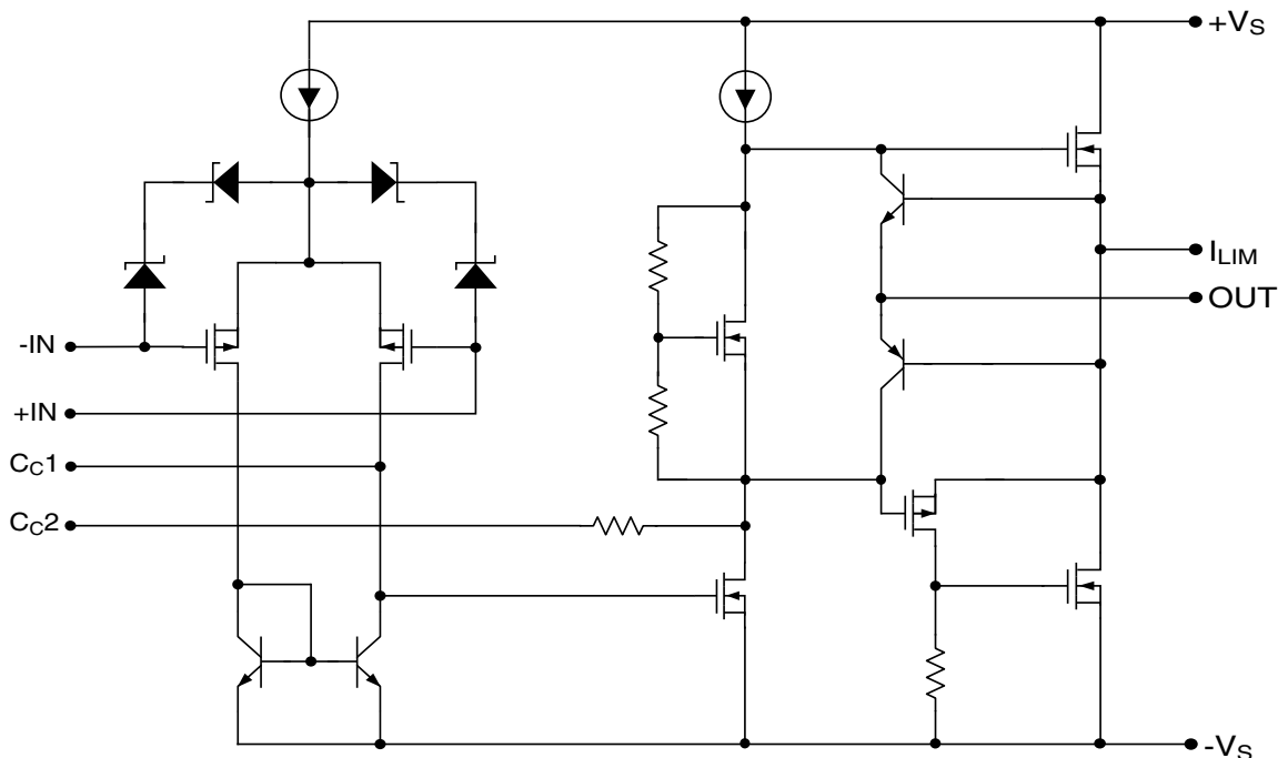
FIGURE 1. Equivalent Schematic
