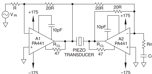
FIGURE 5. Low Cost 660V P-P Piezo Driver
