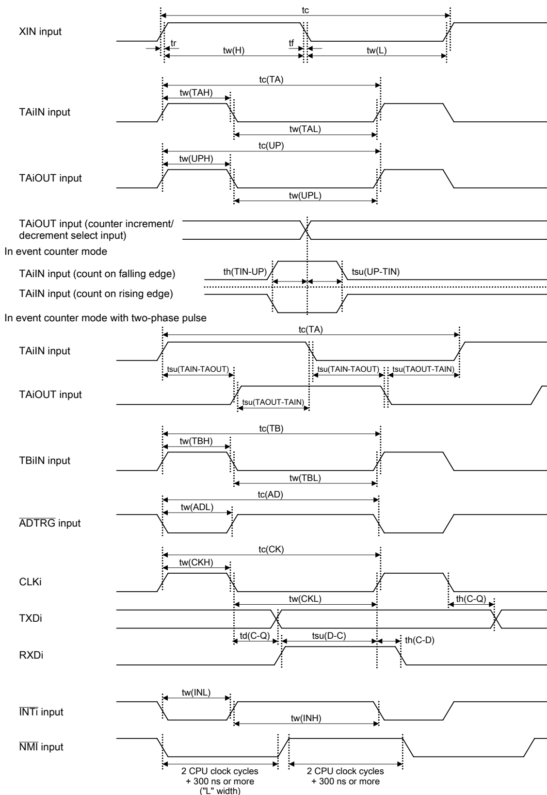
Figure 5.7 VCC1 = VCC2 = 3.3 V Timing Diagram (1)
