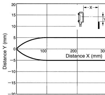
E3T-SR1□ with E39-R4 (Retroreflective)
