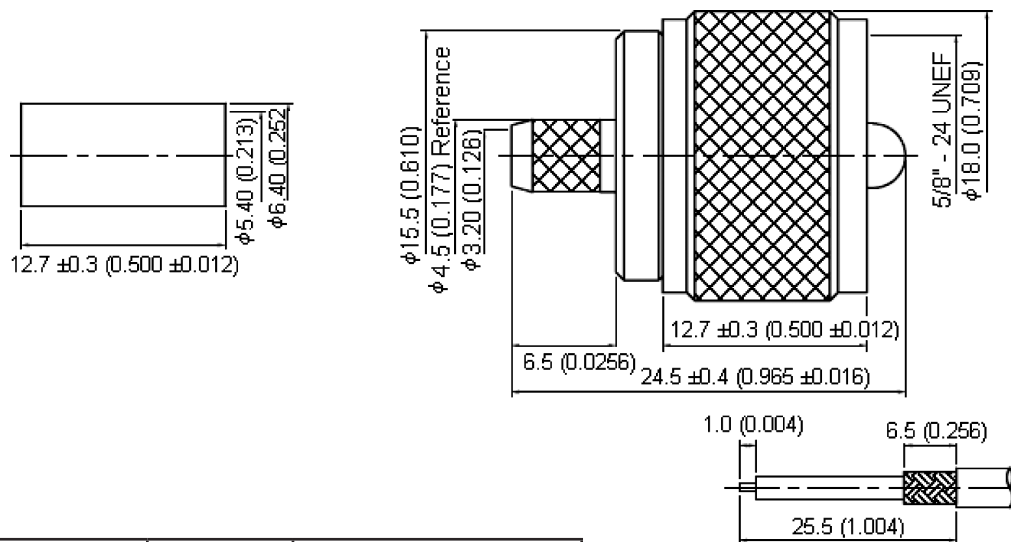
Stripping Dimension
