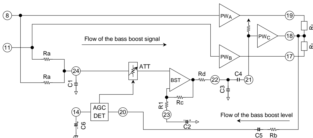
Figure 2 Bass Boost System
