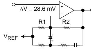
Figure 1 Output DC Voltage of Preamplifier
