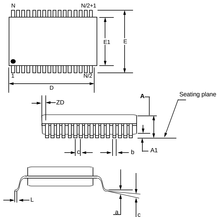
32-pin TSOP 2
