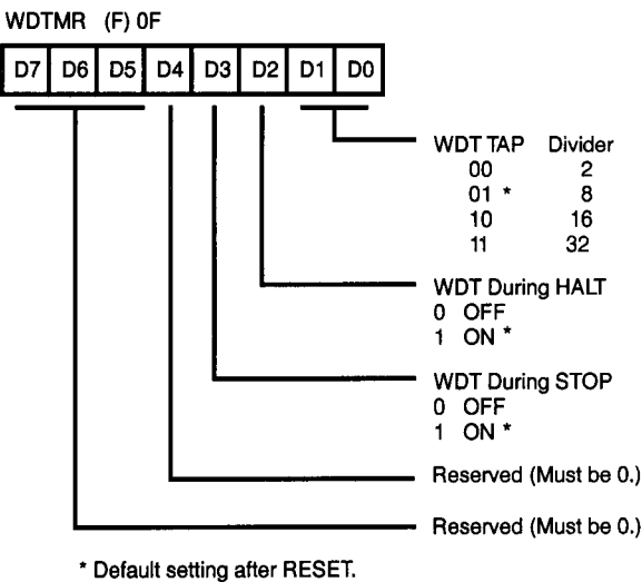
Figure 38. Watch-Dog Timer Mode Register
