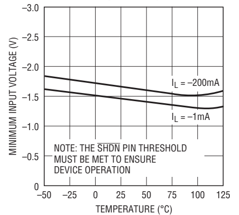
LT1964, LT1964-SD Minimum Input Voltage
