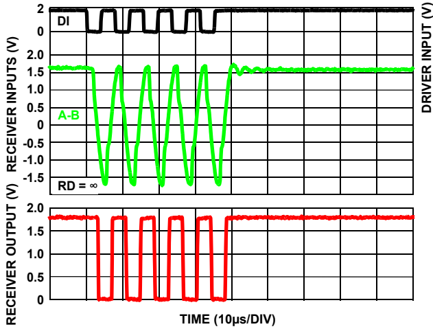
FIGURE 28. ISL32602E, ISL32603E PERFORMANCE WITH V_{CC} = 1.8V , 256kbps, 1000' (305m) CAT 5 CABLE
