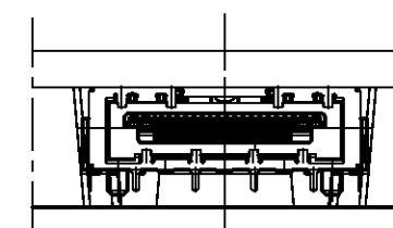
SECT "B"-"B"
