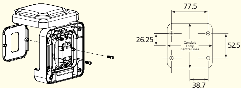
Fixing dimensions
