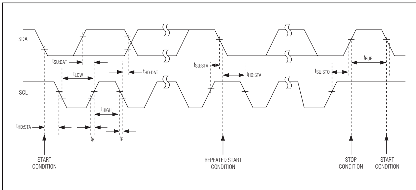
Figure 1. SMBus Timing Diagram
