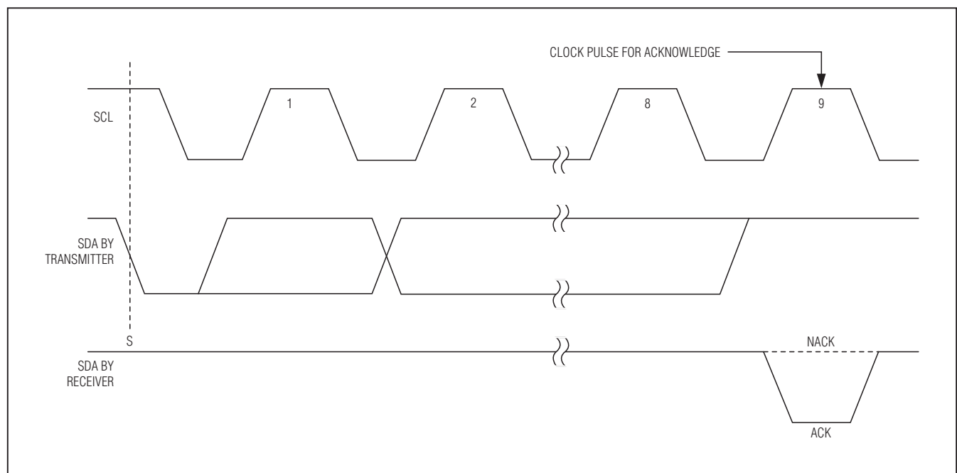
Figure 13. Acknowledge
