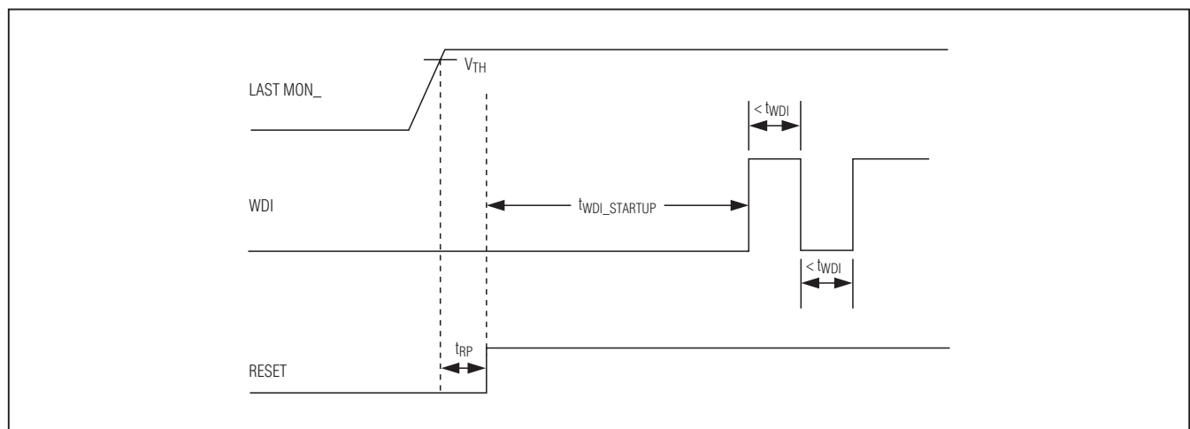
Figure 8. Normal Watchdog Startup Sequence
