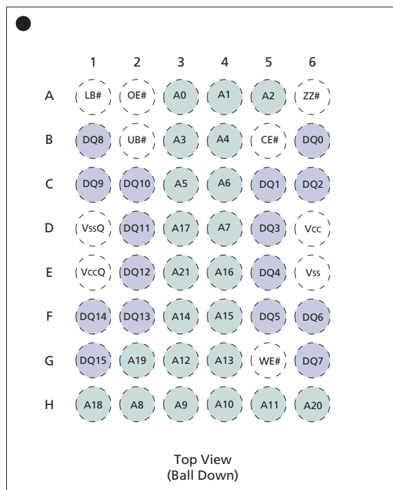
Figure 1: Ball Assignment – 48-Ball VFBGA
