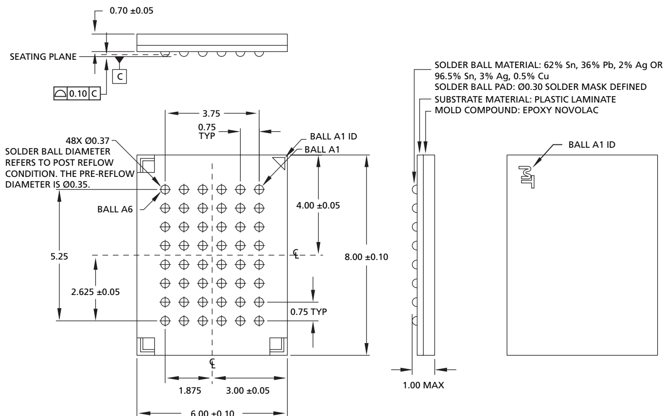
Figure 24: 48-Ball VFBGA
