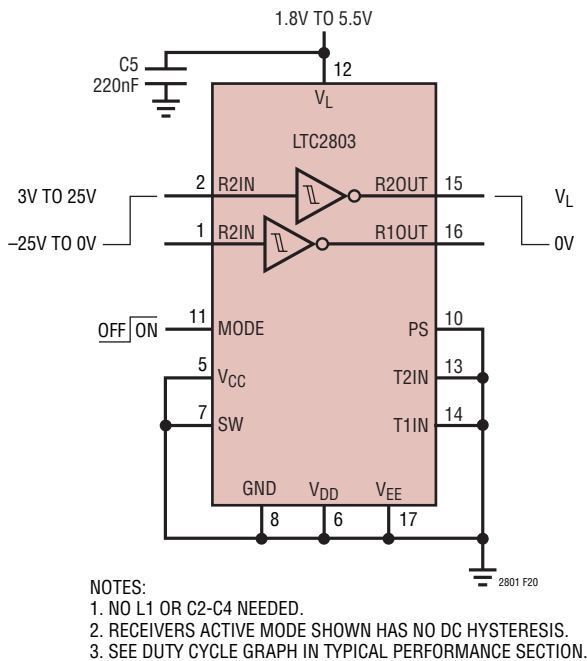
Figure 20. 100kbps Dual Inverting Level Translator ( I_L = 15\mu A Static)
