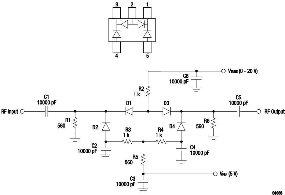
Figure 1. SMP1307-027 Block Diagram and Schematic
