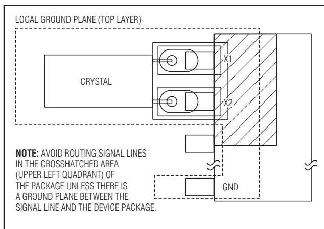
Figure 3. Layout Example
