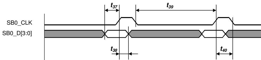
Figure 3.14: Rx Sideband Data Interface; Low Speed Upstream
