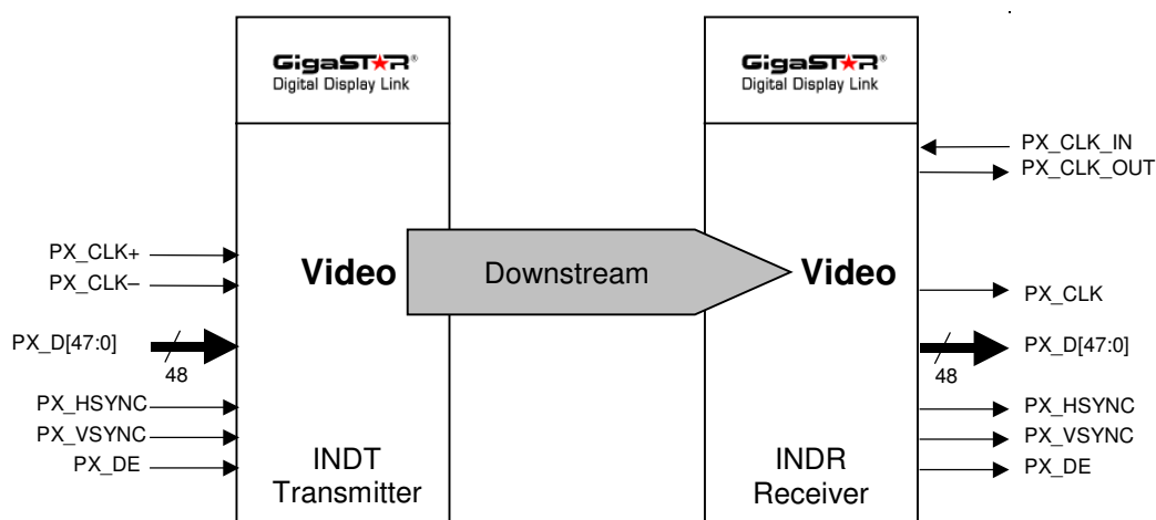
Figure 1.2: Pixel Interface
