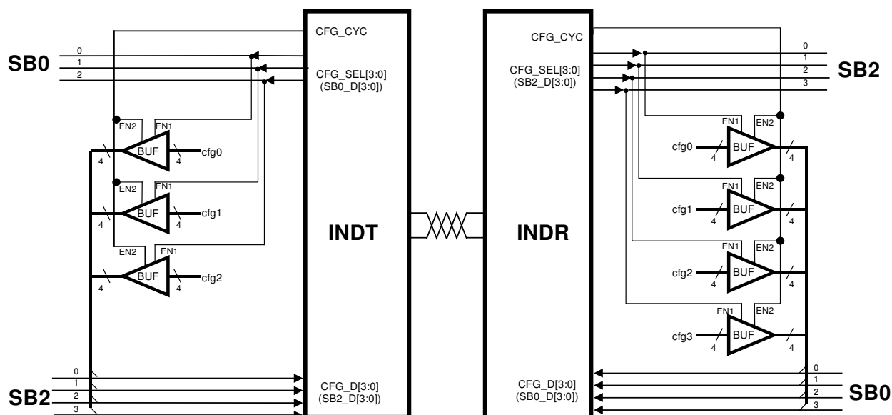
Figure 2.2: Configuration Logic
