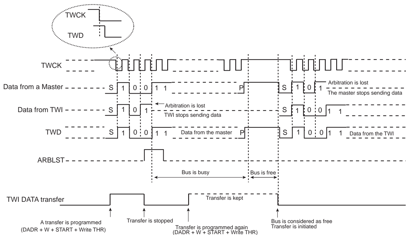
Figure 35-21. Arbitration Cases
