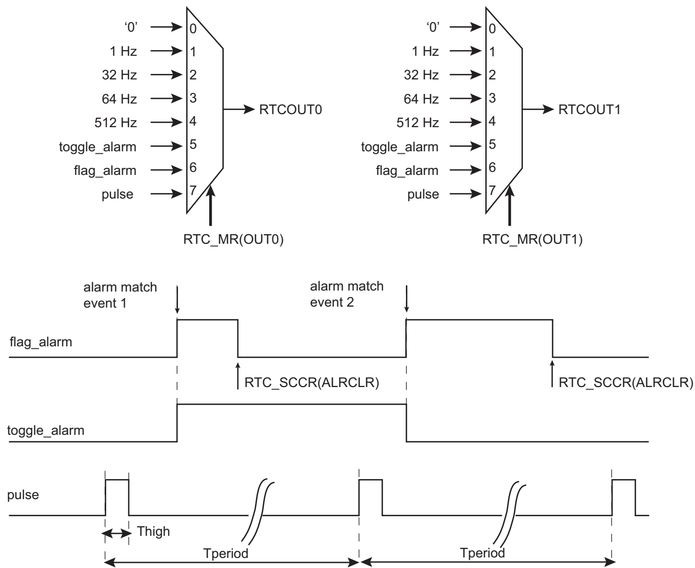
Figure 15-6. Waveform Generation
