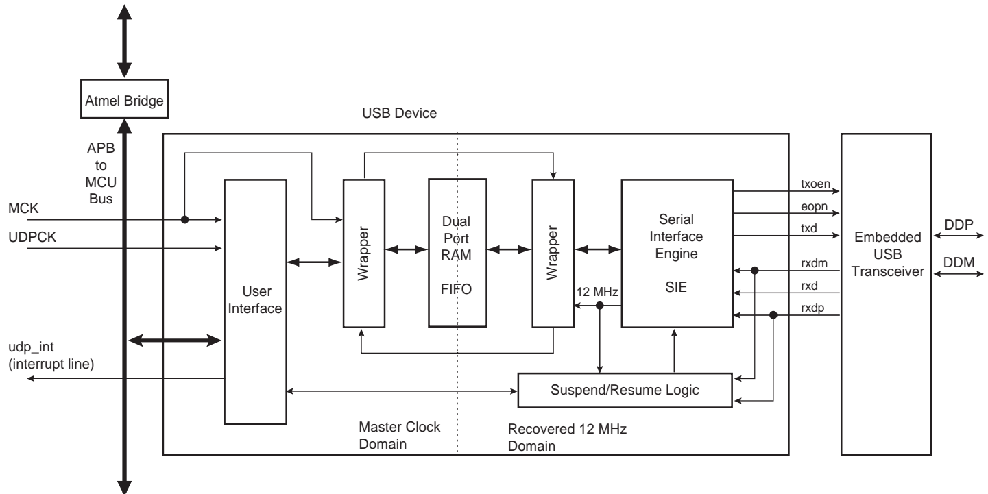
Figure 41-1. Block Diagram
