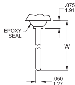
.030(0.76) THK.
