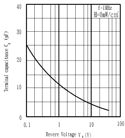
Fig.5 Terminal Capacitance vs. Revere Voltage
