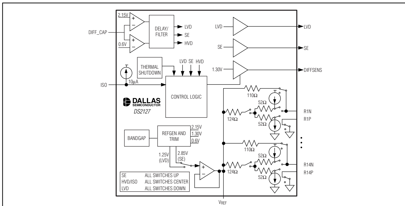
Figure 1. Block Diagram
