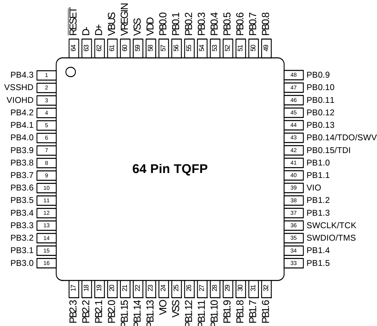
Figure 6.3. SiM3U1x6-GQ Pinout
