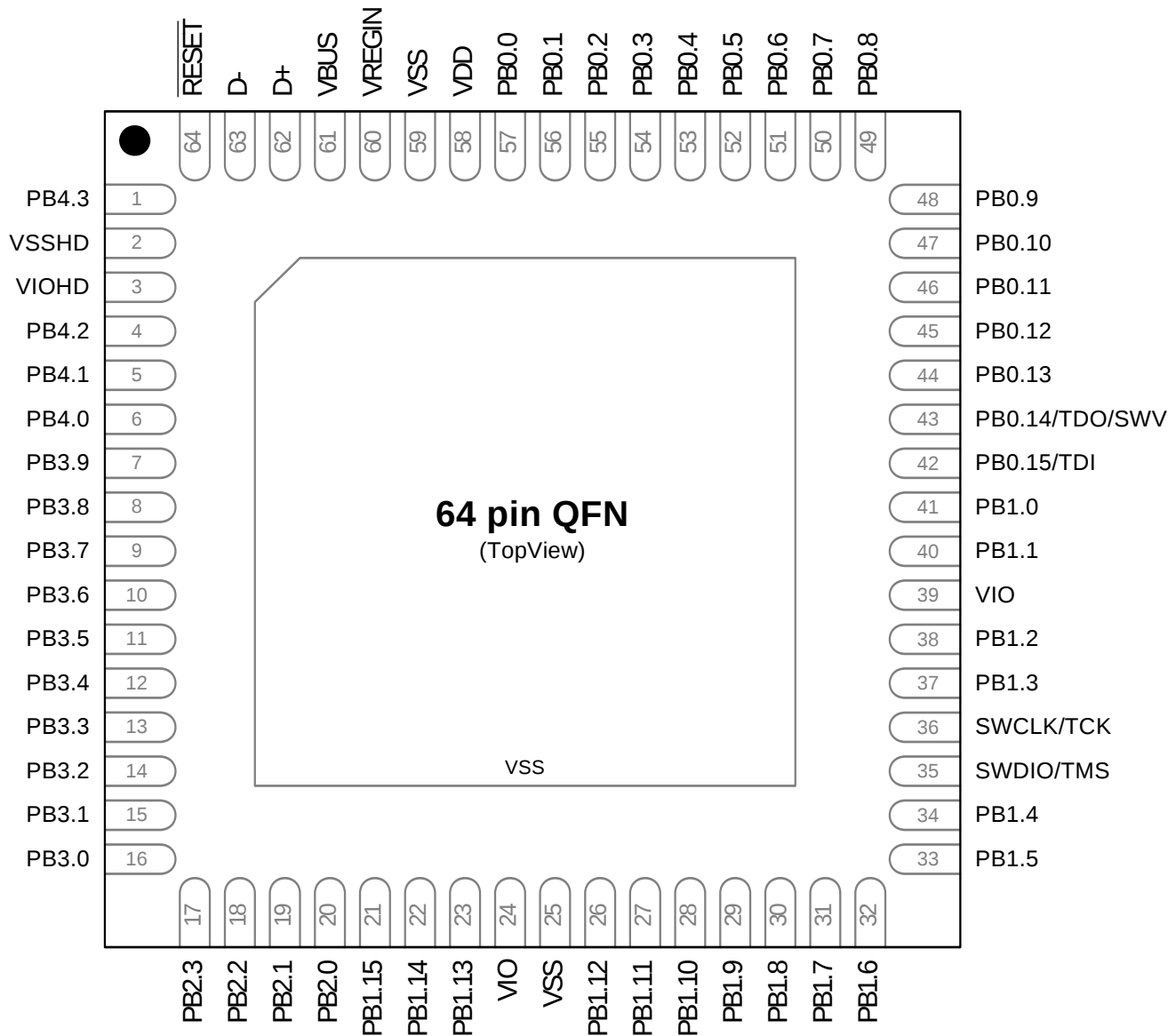
Figure 6.4. SiM3U1x6-GM Pinout
