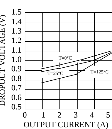
Figure 1. Dropout Voltage vs. Output current
