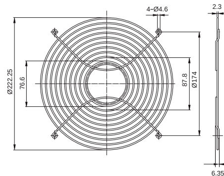
FG-25 For 254mm Fan
