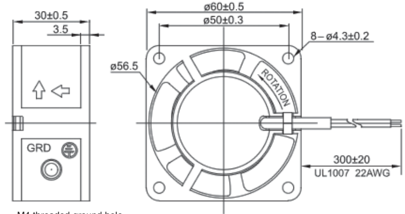
M4 threaded ground hole
