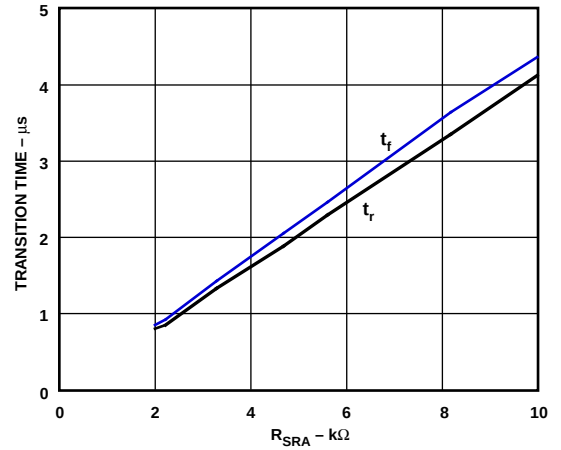
Figure 8. Typical Rise/Fall Times (RS-232 Mode) vs. R_{SRA}
