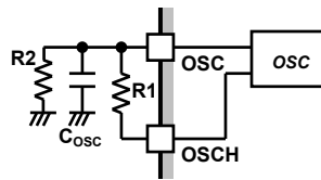
Figure 35. Saw OSC Application
