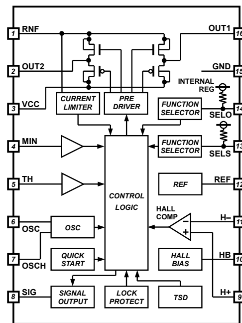
Figure 2. Block Diagram
