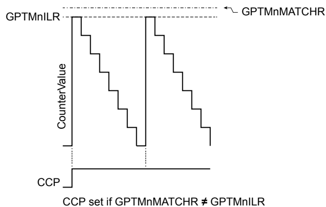
Figure 11-6. CCP Output, \text{GPTMTnMATCHHR} > \text{GPTMTnILR}
