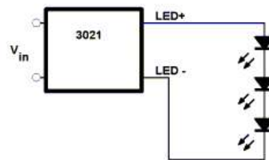
Figure 6. 1000mA unit driving three Luxeon® III emitters ( V_{in} \geq 12VDC )
