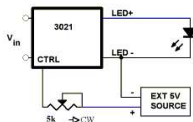
Figure 10. External potentiometer using external voltage source
